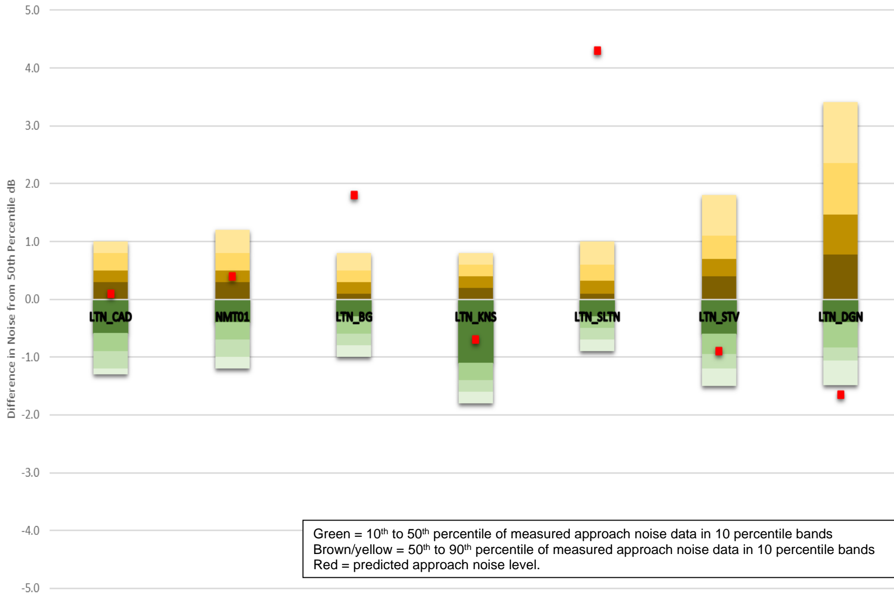
Inset 6.5: A320Neo SEL Approach Noise Testing
