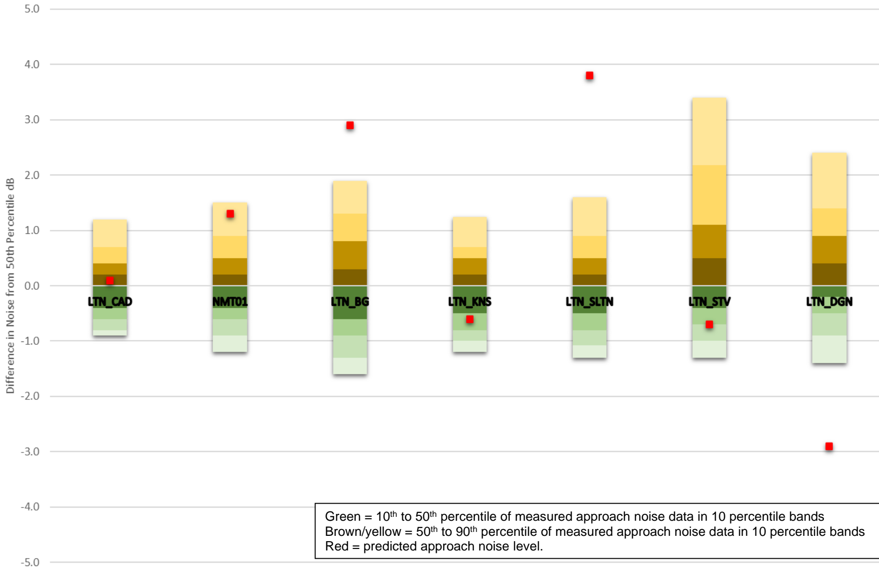
Inset 6.12: A321 L A S max Approach Noise Testing
