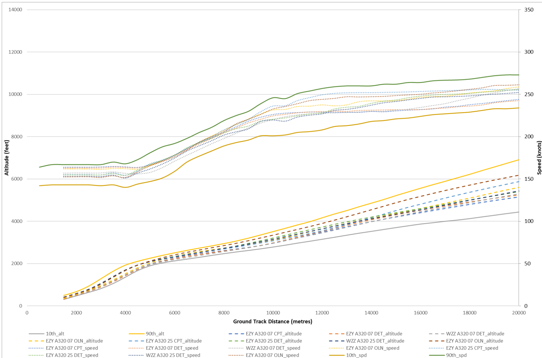
Inset 6.16: A320 Departure Profiles
