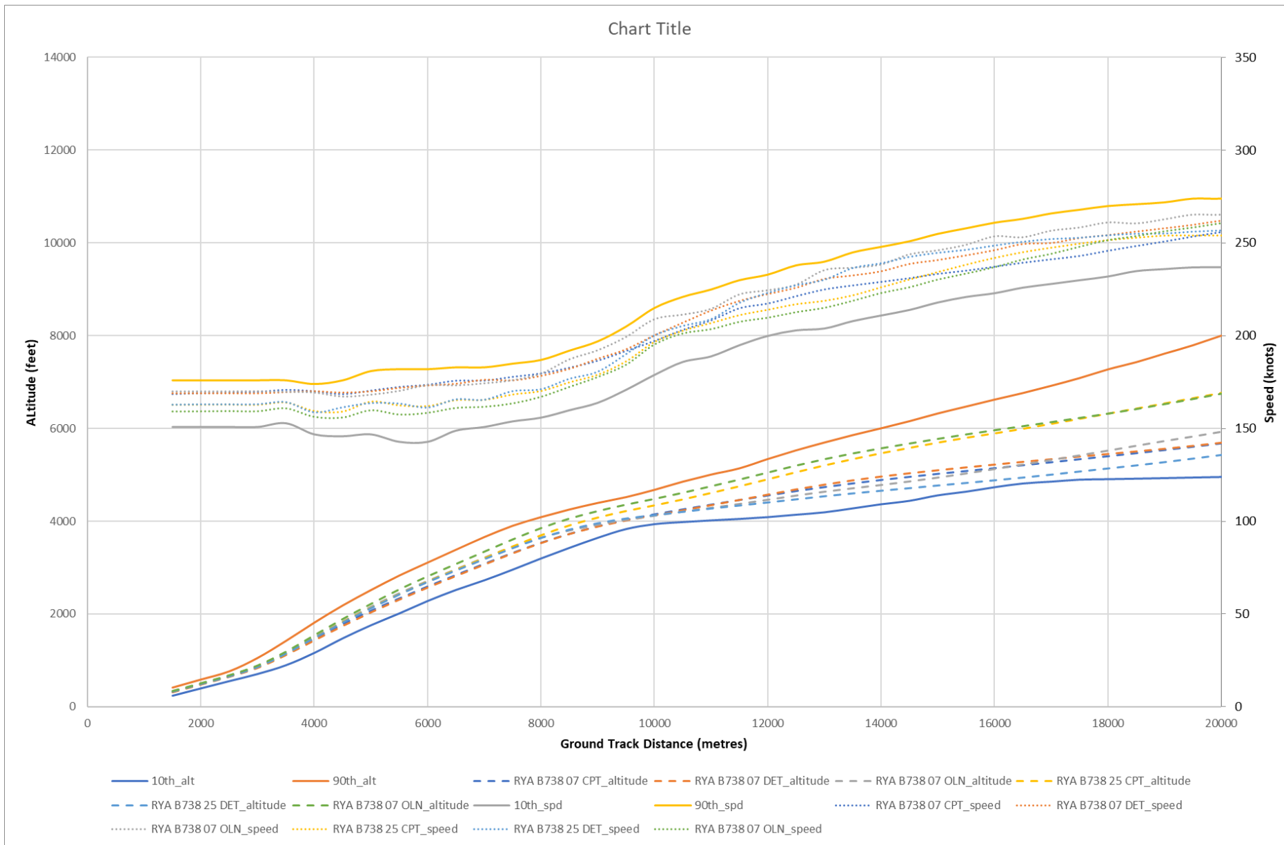
Inset 6.20: B737-800 Departure Profiles
