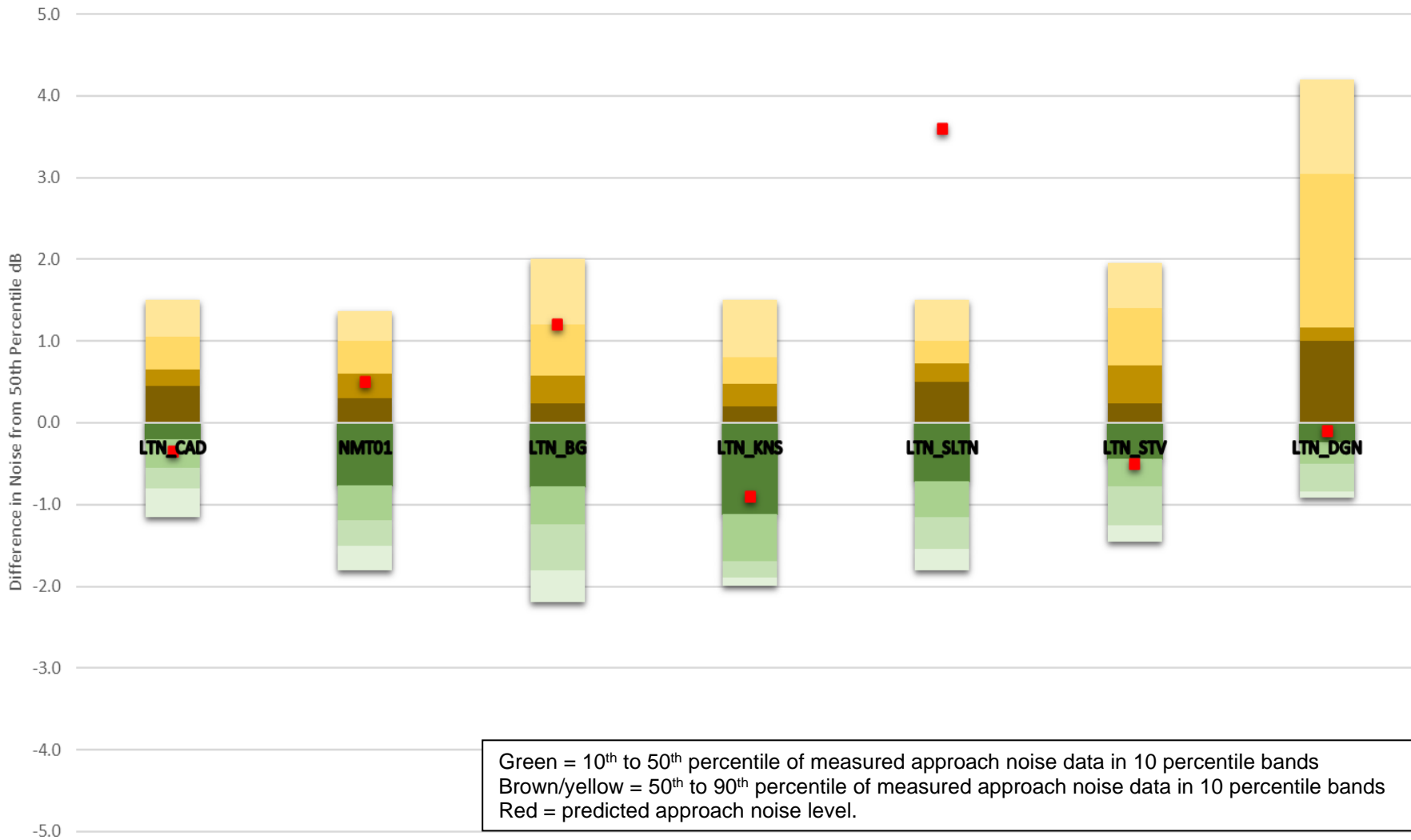
Inset 6.7: A321Neo SEL Approach Noise Testing
